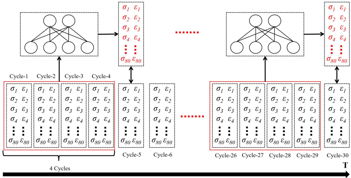
Fig. 5 The schematic diagram of the single-step training and prediction process for LSTM model
