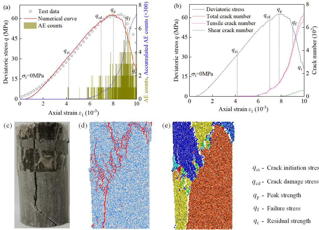
Fig. 3 Comparison the results of laboratory test and numerical simulation
